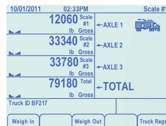
A 32-channel display capability allows viewing of weight on an individual scale and a combination of totalized scales.
